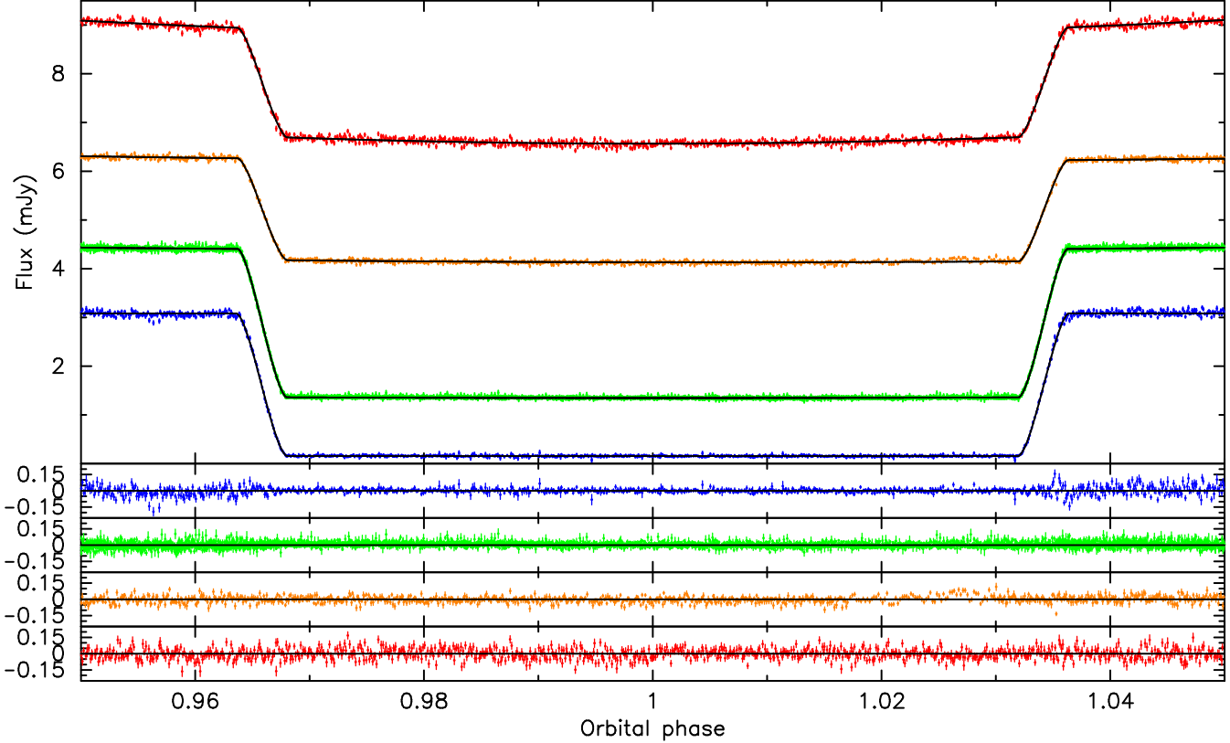
Figure 16. Flux calibrated ULTRACAM u'g'r' and i' band light curves of the eclipse of the white dwarf in QS Vir with model fits overlotted (black lines). We have offset the i' band light curve by -13\text{mJy} to show more detail. The bottom four panels show the residuals of the fit in the u' band (top panel, blue points), g' band (second panel, green points), r' band (third panel, orange points) and the i' band (bottom panel, red points).
