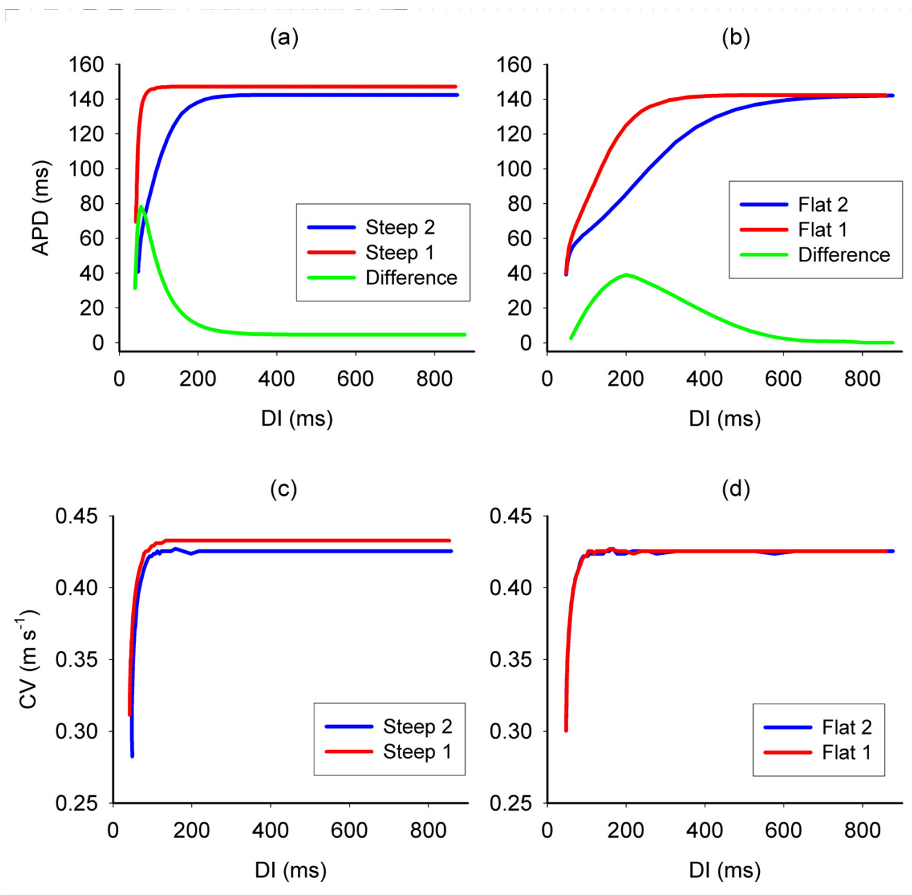
Figure 2 APD and CV restitution measured in a thin strip of uniform tissue. Panels (a) and (b) show APD restitution for the steep and flat variants of the model, and in each case the green line indicates the difference in APD produced at each DI. Panels (c) and (d) show the CV restitution for the steep and flat variants of the model. Model variants with restitution shown in red were allocated to region R1, and those shown in blue allocated to region R2. S3 is blocked in R1, because the tissue is still repolarising from the S2 action potential.
