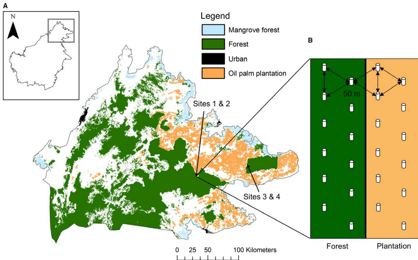
FIGURE 1. (A) Map of Sabah (North Borneo), arrows show study sites. The landcover category ‘forest’ consists of peat swamp forest, lowland evergreen forest, and lower and upper montane forest, and the category ‘oil palm plantation’ shows the extent of mature fruiting oil palm plantations (see Miettinen et al. 2012 for details). (B) Sampling design comprising 24 fruit-baited butterfly traps placed 50 m apart and sampled for a total of 18 d at each site.
