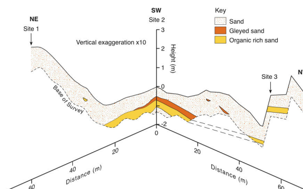
Figure 5: Combined results of the slope profile and auger transects survey from Wangford Warren site 1 to 2 and from site 2 to 3 with heights plotted relative to the ground surface of site 2.
