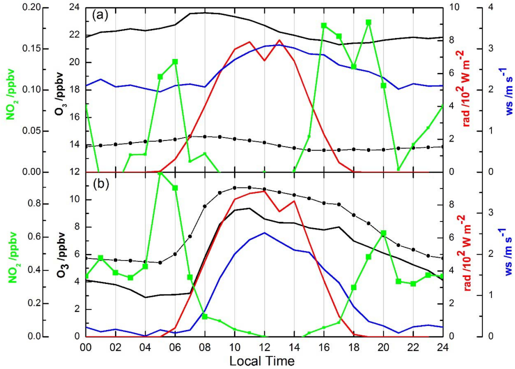
838 Figure 3. Monthly-averaged hourly values of surface O 3 (black), NO 2 (green 839 green squares), global irradiance (red) and wind speed (blue) (the axes titles are color- 840 coded). The large squares represent NO 2 mixing ratios above the detection limit of the 841 instrument. Panel a : monthly averaged daily profiles for October 2010. The average 842 daily profile of O 3 of the two campaigns for September-November is represented by 843 the dotted black line. Panel b : monthly averaged daily profiles for February 2011. The 844 dotted black line represents here the average daily profile of O 3 for February-April.
