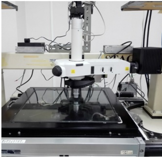
Figure 23: Operational prototype optical microscope systems developed for directional dark matter detection. Left: A system at the Nagoya University. Right: The system used at both Naples and LNGS.
