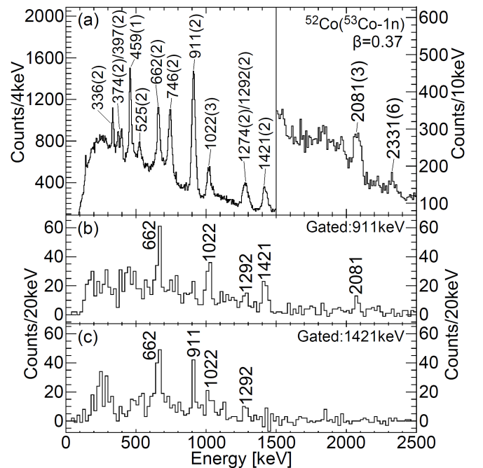
FIG. 2. (a) The Doppler corrected \gamma -ray spectrum for ^{52}\text{Co} fragments, identified following one-neutron knockout from ^{53}\text{Co} . An average \beta_{\text{c}} value of 0.37 was used. (b) and (c) Spectra from a \gamma - \gamma coincidence analysis, on the condition of coincidence with the (b) 911-keV or (c) 1421-keV transition.
