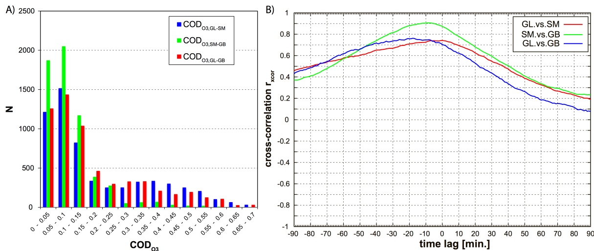
Figure 5. (a) Histogram of the calculated COD O3 values throughout the whole investigation period of HCCT-2010 and (b) calculated cross-correlation ( r_{xcor} ) between the different sites (GL: upwind site; SM: summit site; GB: downwind site) based on measured ozone concentrations for a selected time period (14 September 2010, 11:00 CEST to 15 September 2010, 01:00 CEST).
