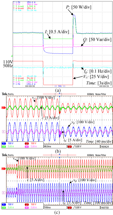
Fig. 10. Operation under grid voltage sag (110 V \rightarrow 55 V): (a) real and reactive power, RMS capacitor voltage and inverter current and grid frequency, (b) transient response when the fault occurs and (c) transient response when the fault is cleared
