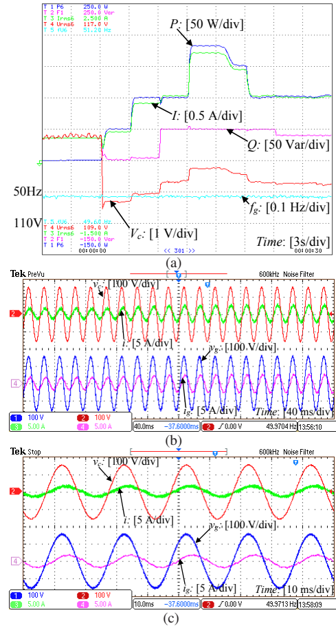
Fig. 6. Operation with a normal grid: (a) real and reactive power, RMS capacitor voltage and inverter current and grid frequency, (b) transient response at t = 15 s (current-limiting property) and (c) steady-state response after 30 s
