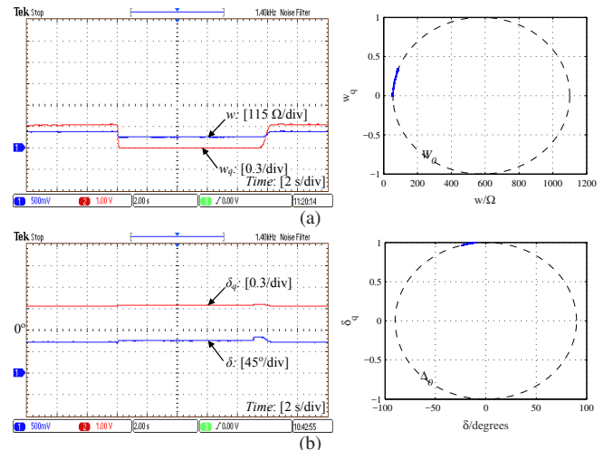
Fig. 9. Transient response of the controller states: (a) w and w_q , and (b) \delta and \delta_q (grid voltage sag 110 V \rightarrow 90 V)
