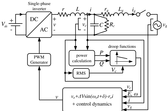
Fig. 3. The overall control system
