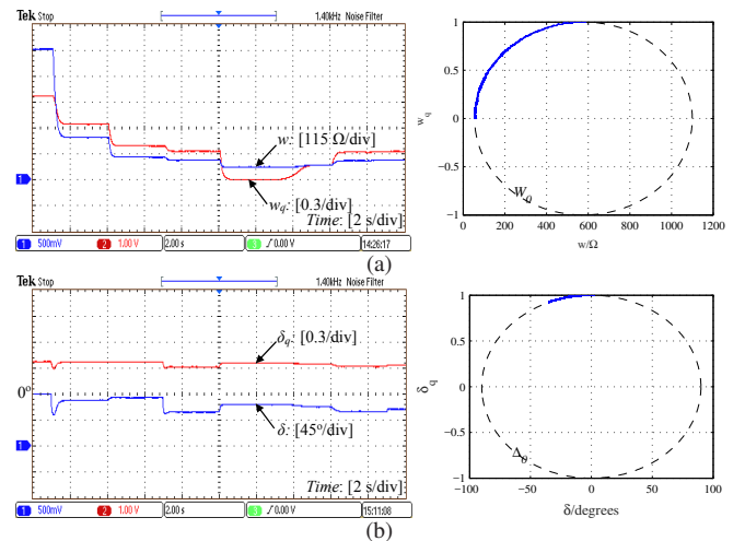
Fig. 7. Transient response of the controller states: (a) w and w_q , and (b) \delta and \delta_q (normal grid)
