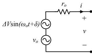
Fig. 2. The equivalent circuit diagram of the controller
