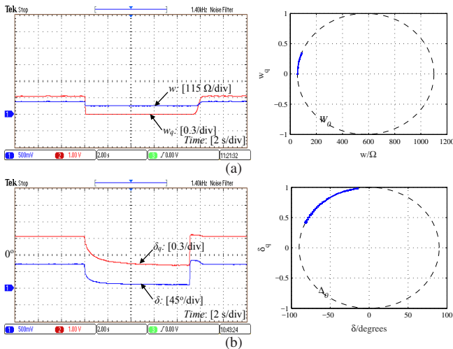
Fig. 11. Transient response of the controller states: (a) w and w_q , and (b) \delta and \delta_q (grid voltage sag 110 V \rightarrow 55 V)
