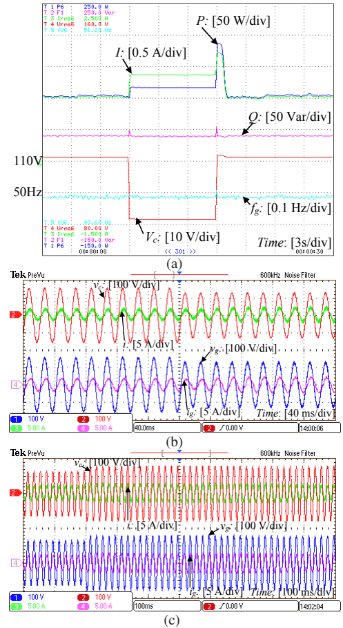
Fig. 8. Operation under grid voltage sag (110 V \rightarrow 90 V): (a) real and reactive power, RMS capacitor voltage and inverter current and grid frequency, (b) transient response when the fault occurs and (c) transient response when the fault is cleared
