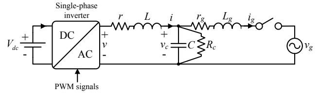
Fig. 1. A grid-connected single-phase inverter with a LCL filter
