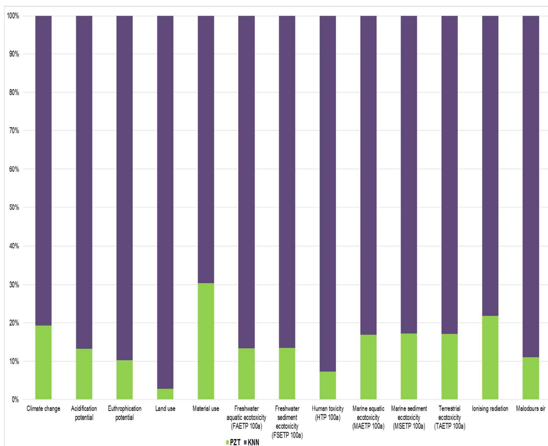
Figure 17: Comparison of environmental profile of PZT versus KNN piezoelectric material (Note: the comparison between KNN and PZT is based on ratio. For instance, the combined impact (process LCA) of the two materials under climate change impact category is 241.11 kgCO 2 -eq with PZT contributing 46.67 kgCO 2 -eq (19%) and KNN 194.45 kgCO 2 -eq (81%). See Supplementary Table S13 for actual data)
