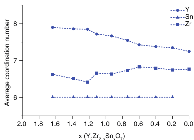
Figure 9. Plot showing the variation in average coordination number of Y, Sn and Zr in the disordered defect fluorite phase as a function of the actual composition (determined from Figure 6(b)). Note, this is not the nominal composition of the starting materials.
