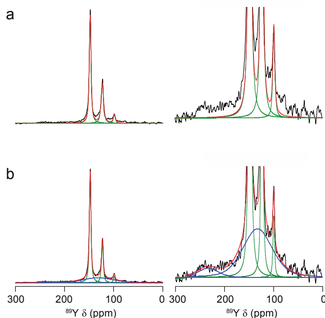
Figure 4. Fits and corresponding (vertical) expansions of the ^{89}\text{Y} MAS NMR spectrum of \text{Y}_2\text{Zr}_{0.2}\text{Sn}_{1.8}\text{O}_7 , shown in Figure 2, (a) without and (b) with broader components (attributed to the defect fluorite phase) included. The green, blue and red lines denote fits for the pyrochlore, defect fluorite and all resonances, respectively.
