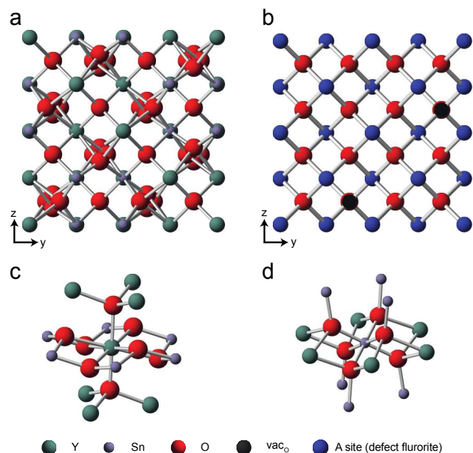
Figure 1. Structure of (a) \text{Y}_2\text{Sn}_2\text{O}_7 pyrochlore and (b) a typical defect fluorite material. Green, small blue and red spheres denote Y ( i.e. , A site), Sn ( i.e. , B site) and O atoms, respectively. In (b), O vacancies are denoted by a black sphere, while the large blue sphere denotes the (single) cation site. Also shown are expansions of the nearest and next-nearest neighbour environments for the (c) eight-coordinated A site and (d) six-coordinated B site in the pyrochlore phase.
