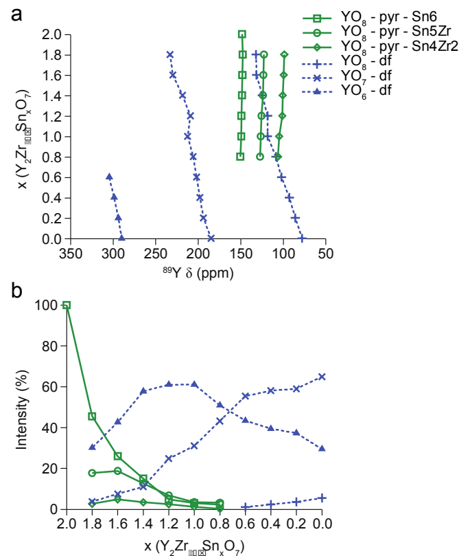
Figure 5. Plot showing the variation of (a) chemical shifts and (b) integrated intensities of the resonances observed in the ^{89}\text{Y} MAS NMR spectra (denoted pyr and df for pyrochlore and disordered defect fluorite phases, respectively) of \text{Y}_2\text{Zr}_{2-x}\text{Sn}_x\text{O}_7 shown in Figure 2, with nominal composition. For the pyrochlore phase, the B-site NNN arrangement for each environment is also shown.
