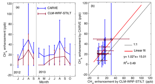
Figure 5. The monthly mean atmospheric mole fraction enhancements in CH 4 estimated by WRF-STILT-CLM4.5 and CARVE measurements. (a) Observed and simulated monthly CH 4 mole fraction enhancements in 2012 and 2013; (b) linear regression of measured versus modeled CH 4 mole fraction enhancements. The error bars are standard deviation of monthly mean.
