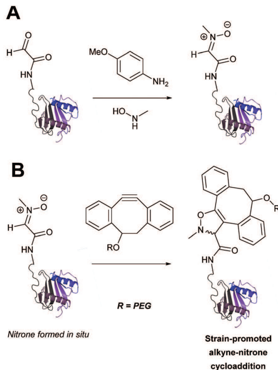
Scheme 11 (A) Glyoxyl-interleukin 8, and formation of a nitronne species. (B) Reaction of an alkyne with the pre-formed nitronne via a cycloaddition.
