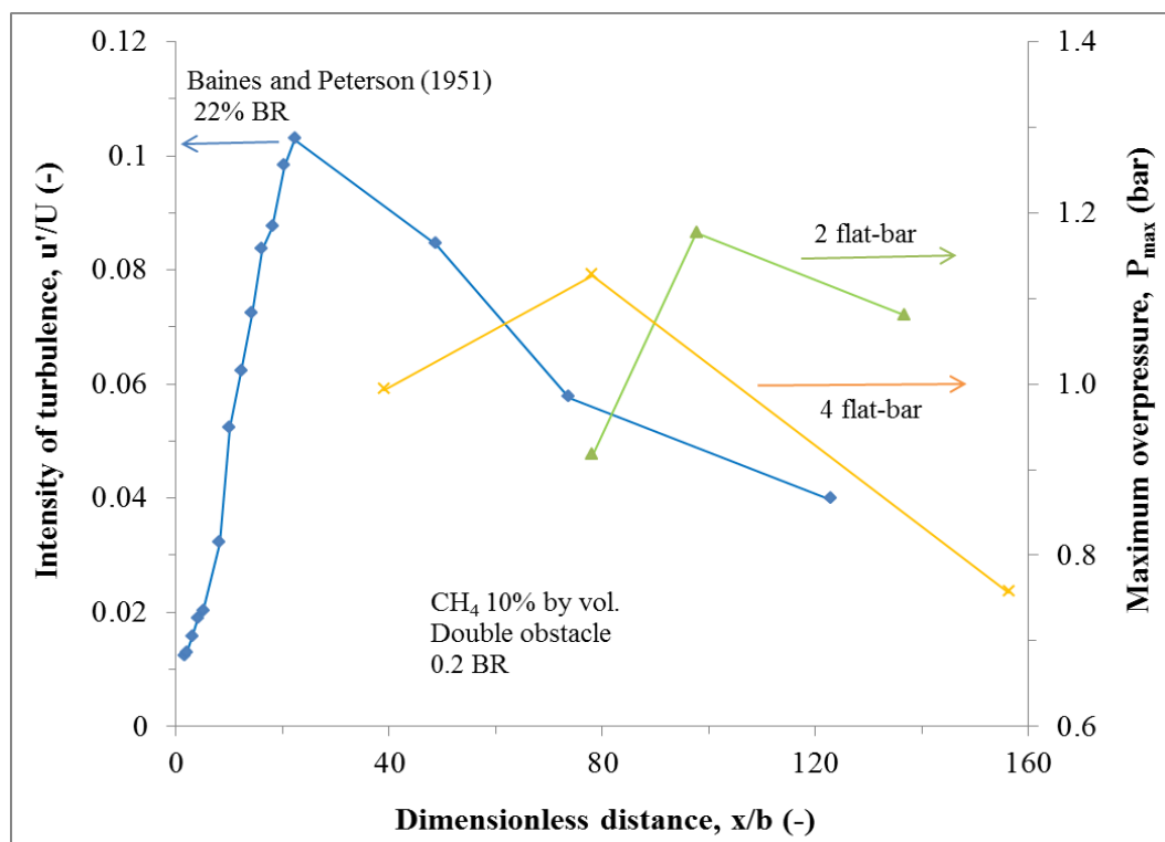
Figure 3: Comparison between intensity of turbulence from cold flow turbulence and transient experimental work with flat-bar obstacles.
