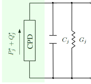
(a) Equivalent circuit scheme for PQ units.
