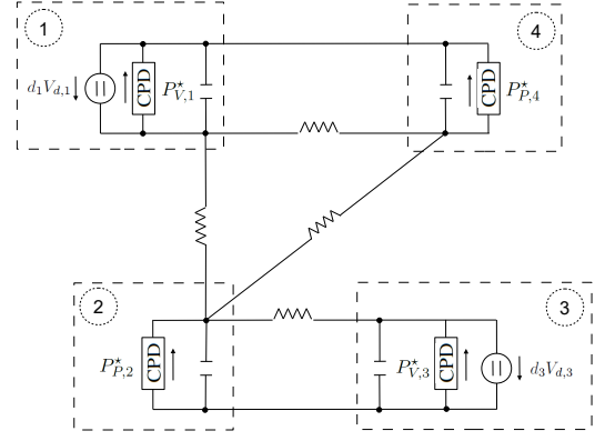
Fig. 2: Four-terminal hvdc transmission system.
