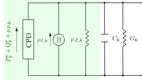
(b) Equivalent circuit scheme for voltage-controlled units.
