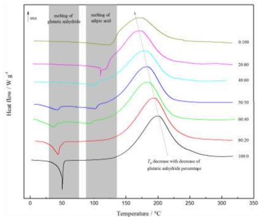
Fig. 1. Thermograms of premixed mixtures of ELO with different compositions of GA:AA at 10\text{ }^{\circ}\text{C min}^{-1} .
