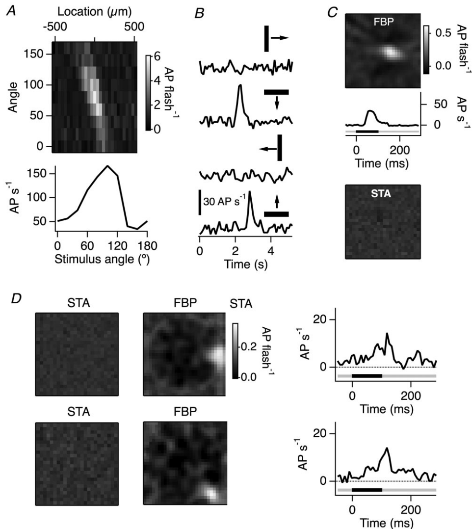
Figure 7. FBP recovers more RFs than STA A, the Radon transform over 9 angles is shown on top for an orientation-selective cell. The peak response vs. the angle of the bar is shown below. The response is strongest for angles around 90 deg. B, the same cell responding to a bar moving in 4 different directions. No response is seen for bars moving at either 0 or 180 deg, but clear responses are seen for bars moving along 90 or 270 deg. C, the RF of the cell recovered with the FBP and the STA methods. Note that the RF is not apparent in the STA image. The temporal component measured with FBP is shown below. D, two examples of cells with weak responses that were recovered by the FBP method but not by the STA method with their temporal responses shown to the right.
