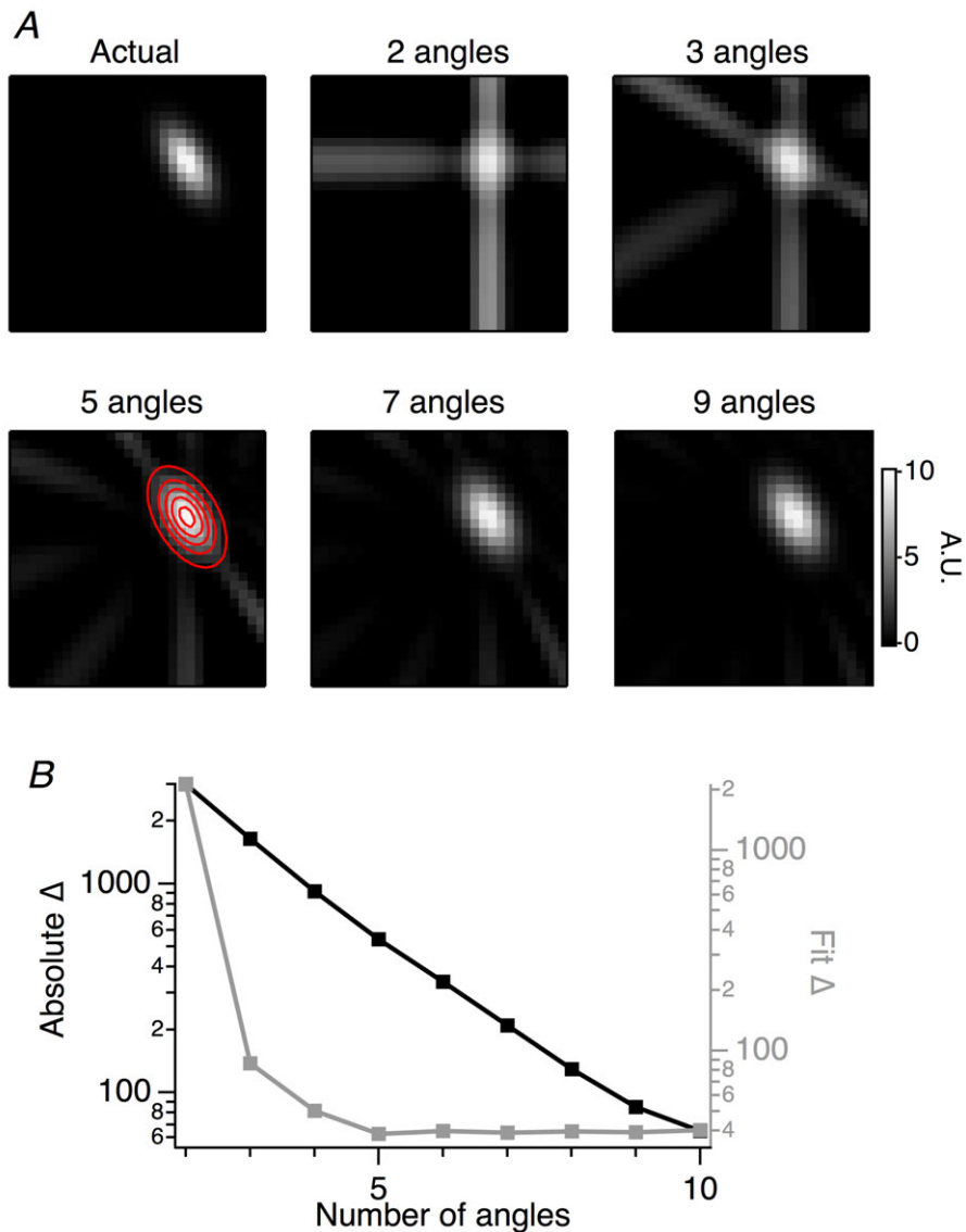
Figure 3. Five angles for the Radon transform are sufficient to reconstruct the RF A , Radon transforms, using different numbers of angles, were taken of the model RF (Actual). These transforms were then used with FBP to reconstruct the RFs shown (2–9 angles). With more angles, we achieve finer resolution and closer likeness to the original image. The red contours shown on 5 angles is a 2-D Gaussian fit to the reconstructed RF. B , comparison of the quality of reconstruction with different numbers of angles. Plotted in black are the absolute differences in pixel value between the reconstruction and the original model. Note that the difference between the reconstructed image and the original decrease with increasing angles. Plotted in grey is the absolute difference between a 2-D Gaussian fit to the reconstruction and the original model. Note that 5 angles are sufficient to capture the centre, size and shape of the object.
