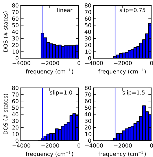
FIG. 7: Density of states for A = 3 and various values of s . The bin size is 200 \text{ cm}^{-1} .
