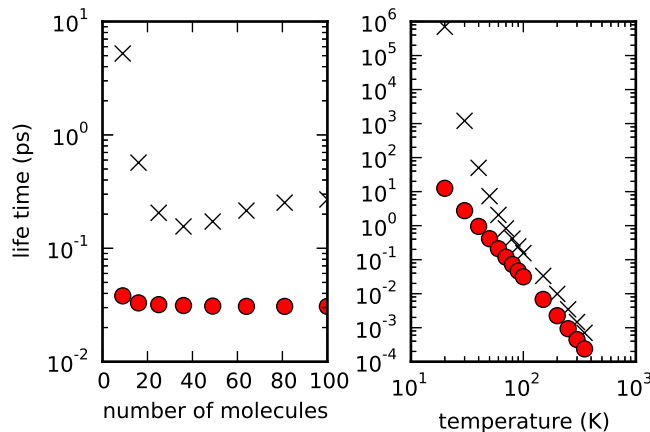
FIG. 4: Calculated intraband scattering life time of the bright exciton state with the model of Heijs et al. in an N \times N brick layer lattice (crosses, A = 2 , s = 1 ) and an N^2 \times 1 linear chain (circles) (left) as a function of the system size ( N^2 ) at a temperature of 100 K and (right) as a function of temperature for N = 6 . The coupling in the x-direction is J = -500\text{cm}^{-1} .
