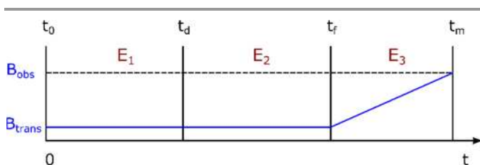
Figure 3. The variation of magnetic field in the SABRE experiment as a function of time. E_1 , E_2 , and E_3 denote three evolution periods during the time intervals ( t_0 - t_d ), ( t_d - t_f ), and ( t_f - t_m ) respectively. B_{trans} and B_{obs} represent transfer and observation magnetic field strengths respectively.
