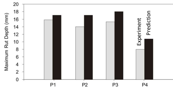
Figure 2. Comparison between rut depths measured at 36 months and numerical predictions.
