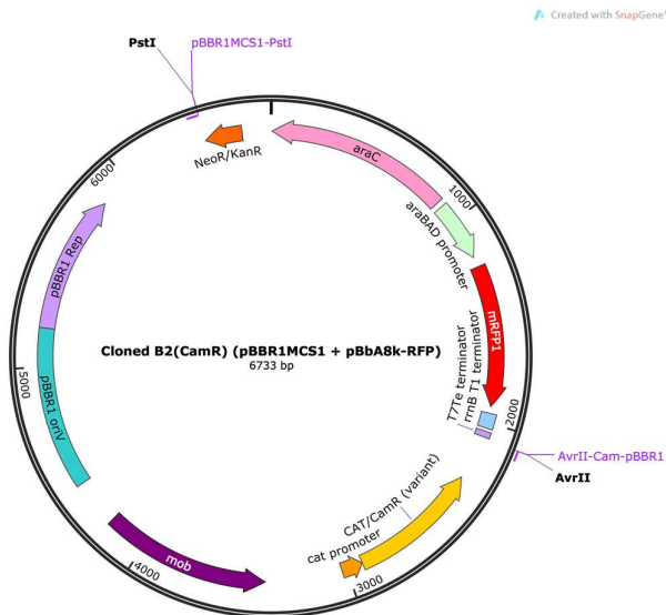
Figure 2. Plasmid B2(CamR).
