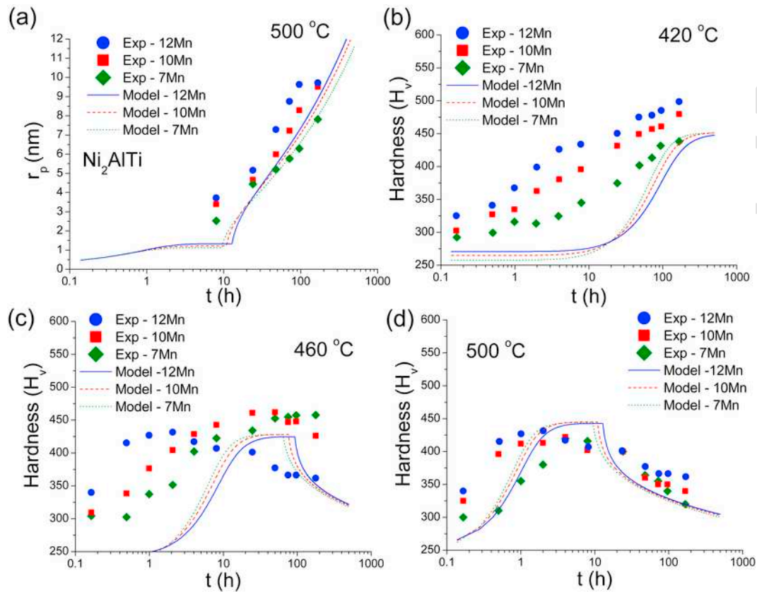
Fig. 5. Results on intermetallic formation and strengthening in Lean7Mn, Lean10Mn and Lean12Mn. (a) particle radius, and hardness evolution at (b) 420 °C, (c) 460 °C, (d) 500 °C.
