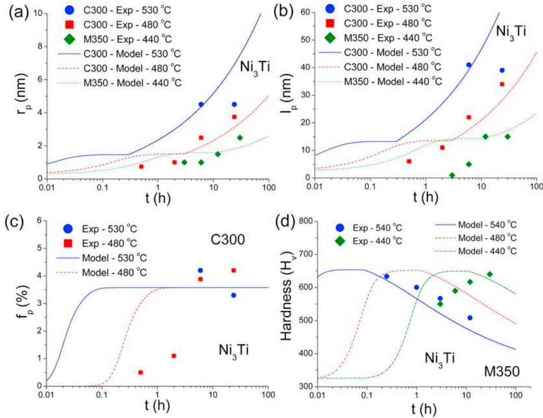
Fig. 6. Results on Ni 3 Ti formation and strengthening in C300 and M350: (a) particle radius and (b) length; (c) phase fraction evolution, and its (d) corresponding hardness.
