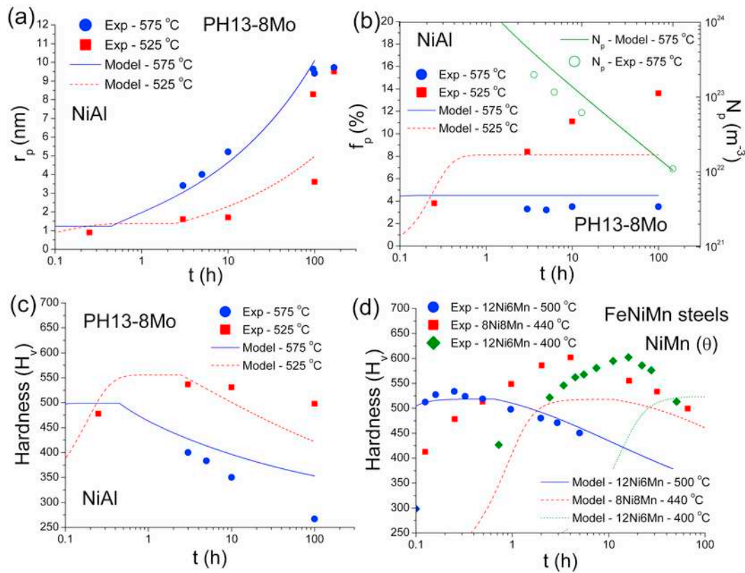
Fig. 4. Results on intermetallic formation and strengthening in PH13—8Mo: (a) mean particle radius, (b) volume fraction and number density and (c) hardness evolution. (d) Hardness evolution in \theta -containing Fe—Ni—Mn steels.
