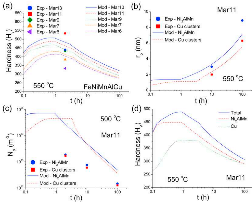
Fig. 9. Strengthening analysis when multiple precipitation occurs in Fe—Mn—Ni—Al—Cu. (a) Variations in the hardness for various compositions; (b) mean particle radius and (c) number density in Mar11. (d) Individual strengthening contribution in Mar11 from Ni_2AlMn and Cu precipitates.
