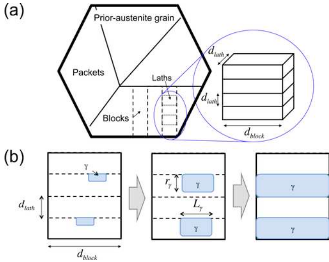
Fig. 1. (a) Schematic representation of the hierarchical structure of lath martensite with laths of cuboidal morphology. (b) Mechanism of austenite reversion in lath martensite.
