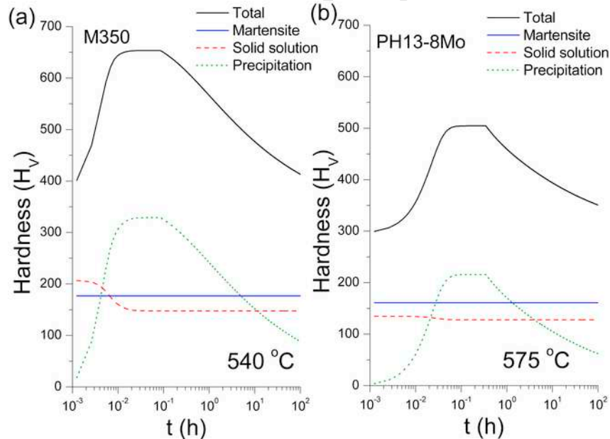
Fig. 7. Relative contribution to strengthening in (a) M350 and (b) PH13-8Mo.
