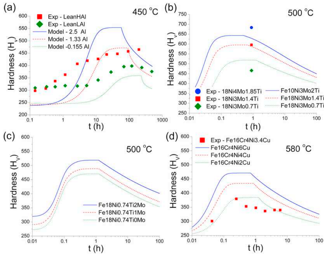
Fig. 8. Analysis on the hardness variations with alloying content. (a) Al effects in Fe-2Ni-10Mn-1Mo-Al; (b) Ti effects in Fe-18Ni-3Mo-Ti; (c) Mo effects in Fe-18Ni-0.74Ti-Mo; and (d) Cu effects on Fe-16Cr-4Ni-Cu.
