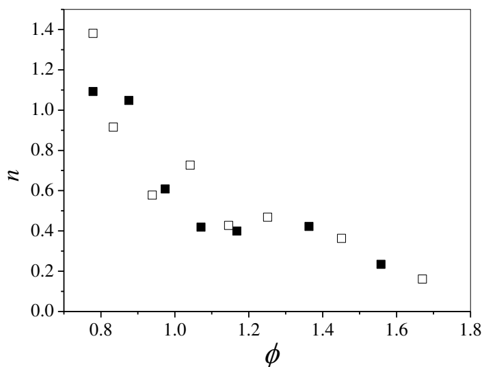
Figure 12. Values of the exponent, n where u_{te} \propto u_l^n . Filled symbols, u' = 2 m/s; open symbols, u' = 6 m/s.
