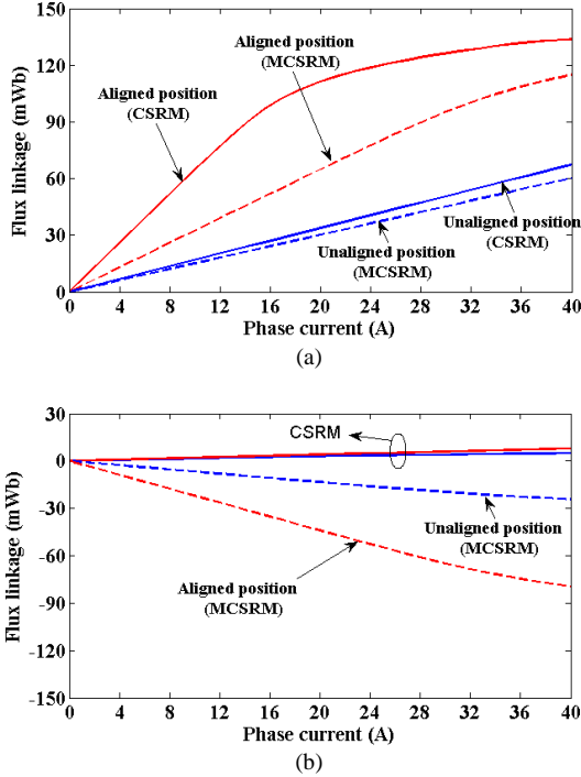
Fig. 3 Self and mutual flux linkages vs phase current for different rotor positions of CSRMs and MCSRMs. The phase A supplied by dc current and the mutual flux linkage is captured by phase B. (a) self flux linkage, (b) mutual flux linkages.
