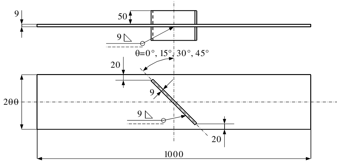
Out-of-plane gusset specimen
