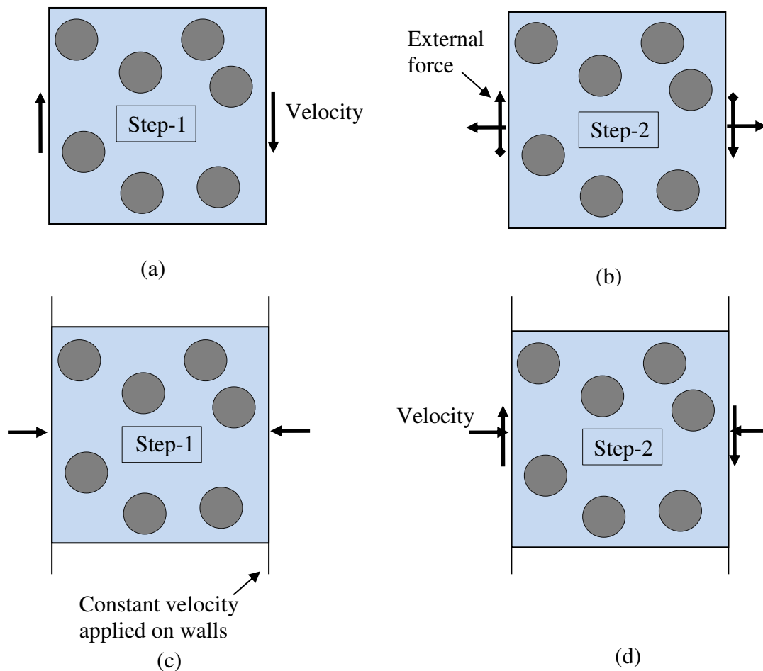
Fig.17 Loading schemes used to perform biaxial tests (arrows \blacktriangleleft\blacktriangleright represent external force and arrows \rightarrow represent velocity applied): (a)-(b) shear and tension in Part-A, and (c)-(d) shear and compression in Part-B.
