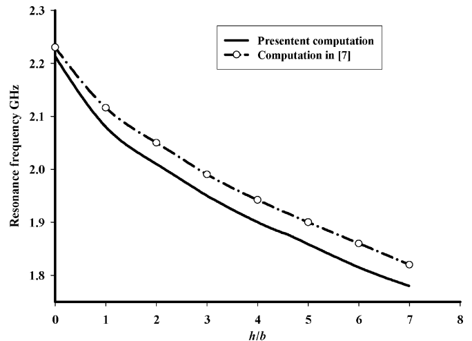
Fig. 7. The resonance frequency of a spherical circular microstrip antenna as a function of superstrate thickness.
