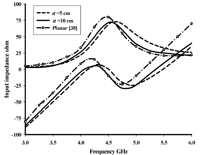
Fig. 9. Input impedance of a proximity coupled spherical rectangular patch antenna.
