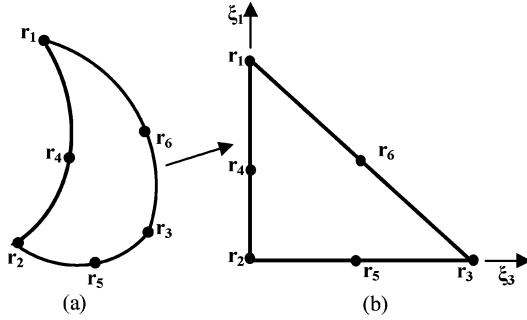
Fig. 2. (a) Curvilinear triangle in the Cartesian coordinates. (b) Equivalent planar triangle in the parametric coordinates \xi_1 , \xi_2 and \xi_3 .
