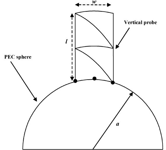
Fig. 3. A monopole strip attached to a PEC sphere.
