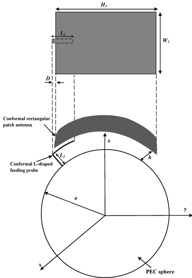
Fig. 8. A spherical rectangular patch antenna proximity fed by a conformal L-shaped probe.
