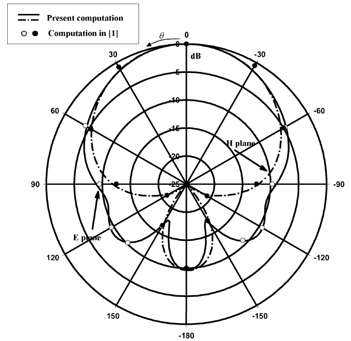
Fig. 6. Radiation pattern of a spherical circular microstrip antenna.
