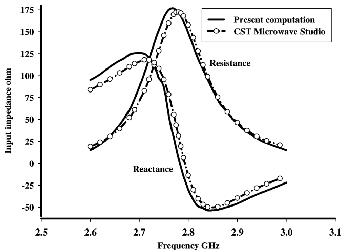
Fig. 5. The input impedance of a spherical circular microstrip antenna.
