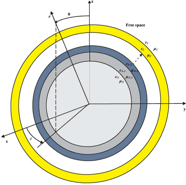
Fig. 1. A layered dielectric sphere.
