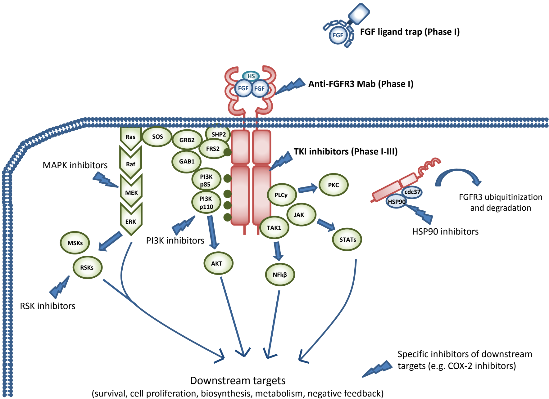
Figure 4. Signalling pathways activated by FGFR3 and potential therapeutic approach to targeted inhibition. In bold, FGFR-specific inhibitors and current clinical trial phase.
