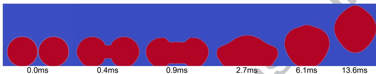
Figure 7: Results of 2D LB modelling of droplet coalescence and jumping phenomenon, initial droplet radius 405\ \mu\text{m} and droplet velocity \bar{v}_j = 0.064\ \text{m/s} .
