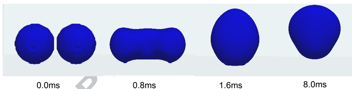
Figure 8: Results of 3D VOF modelling of droplet coalescence and jumping phenomenon, initial droplet radius 405\ \mu\text{m} and droplet velocity U = 0.082\ \text{m/s} .
