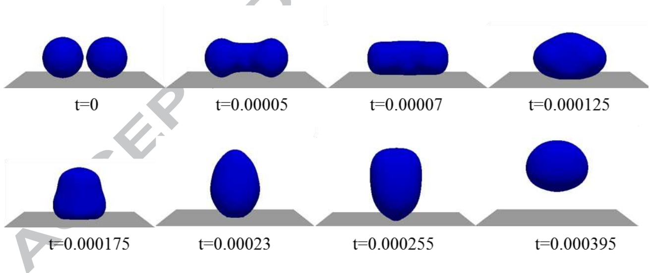
Figure 4: Time sequence of the 3D coalescence of two droplets ( x - y view) with initial radius r = 75\mu\text{m} and static angle \theta_s = 180^\circ . The isosurface \alpha=0.5 is displayed.
