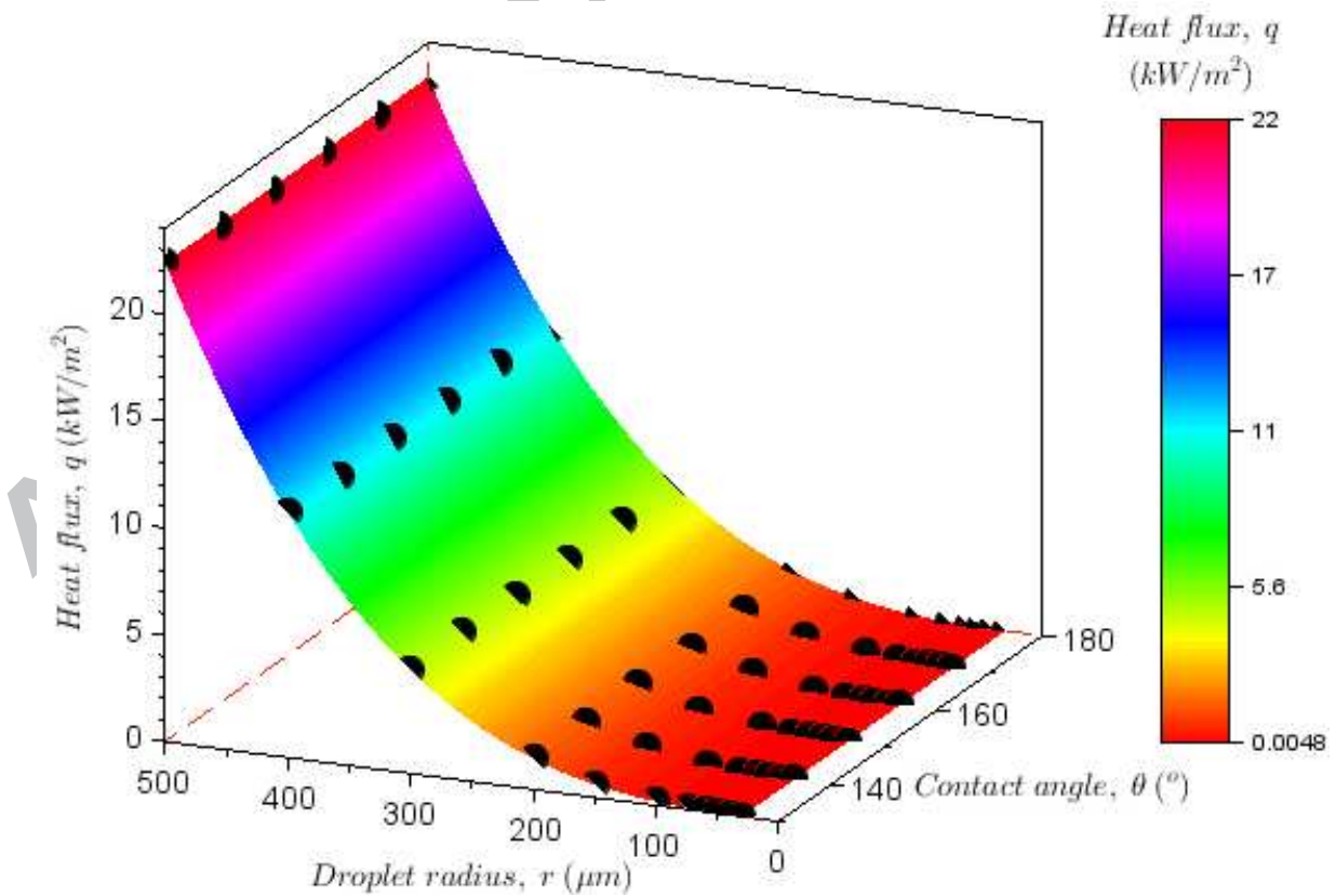
Figure 12: Response surface of the heat flux q together with the DOE points; ●.
