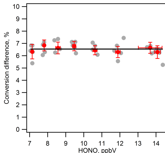
Figure 2. Difference in HONO conversion between 385 and 395 nm UV-LEDs over a range of dilutions. Median values are in red, whilst all data are shown in grey. Linear fit is in black; error bars show standard deviation of the mean values.
