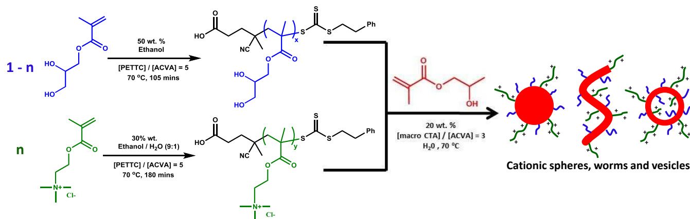
Figure 1. Synthesis of cationic diblock copolymer nanoparticles with the general formula [(1-n) \text{ PGMA}_x + [n] \text{ PPDMA}_y] - \text{PHPMA}_z by RAFT aqueous dispersion polymerisation of HPMA using a binary mixture of non-ionic and cationic macro-CTAs. Optimisation of n , x , y , and z enable the formation of cationic spheres, worms or vesicles.
