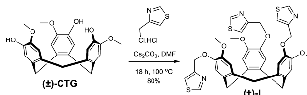
Scheme 1 Synthetic route to (±)-tris-(4-methylthiazolyl)cyclotrighuaiacylene.
