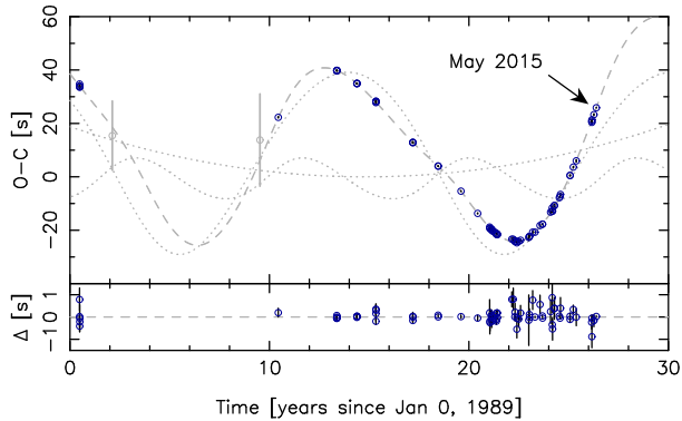
Figure 7. O-C diagram of NN Ser. The dashed line indicates the best fit model, which includes two circumbinary Jovian planets as well as a quadratic trend with a much longer period (dotted lines). The lower panel shows the residuals with respect to the best fit.
