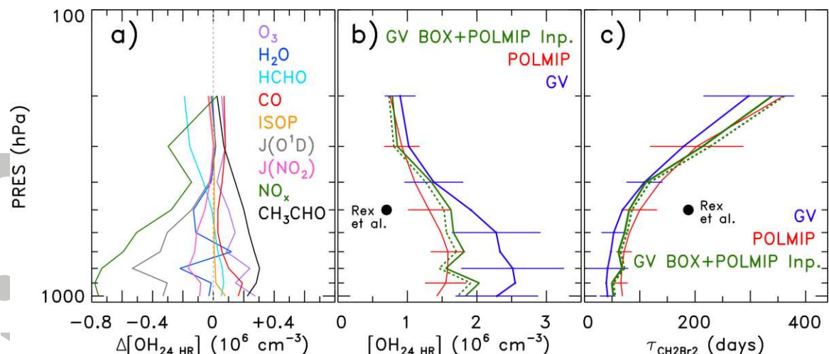
Figure 10. Panel a) shows the difference in [OH] 24 HR between a run of the DSMACC box model constrained to GV observations of all OH precursors with the exception of the indicated species and another run of the model constrained to GV observations of all OH precursors, where indicated species refers to the POLMIP multi-model mean value. These box model difference plots have been conducted at 100 hPa intervals. Panel b) shows the mean and standard deviation [OH] 24 HR profile calculated by the DSMACC box model constrained to GV observations of OH precursors (blue) compared to the multi-model mean and standard deviation of monthly mean [OH] in the POLMIP archive from eight CTMs (red). The solid green line represents [OH] 24 HR CONTRAST (blue) + Δ[OH] 24 HR ALL , where Δ[OH] 24 HR ALL represents the difference between a run of the DSMACC box model constrained to POLMIP multi-model mean values of all nine OH precursors and another run of the model constrained to GV observations of all nine OH precursors. The profile of Δ[OH] 24 HR ALL is nearly identical to the sum of the nine terms shown in panel a) (see supplement). The dashed green line is adjusted to account for the 13% high bias in daytime OH calculated by the box model, or ~6.5% high bias in OH 24 HR , attributable to the box model chemical mechanism (from Figure 5d). The calculation of the dashed green line is identical to the solid green line except that values of [OH] 24 HR are multiplied by 1 / 1.065 . Panel c) shows lifetime of CH 2 Br 2 (τ CH 2 Br 2 ) with respect to loss by OH for [OH] 24 HR from the box model constrained to GV measurements (blue), for the multi-model monthly mean [OH] from the POLMIP CTMs (red), and for [OH] 24 HR from the box model constrained to the nine OH precursors from POLMIP (solid green). The dashed green line in panel c) shows τ CH 2 Br 2 calculated for adjusted values of [OH] 24 HR in panel b) represented by the green dashed line. Values of [OH] 24 HR and τ CH 2 Br 2 reported by Rex et al. [2014] at 500 hPa for October 2009 in the TWP are shown in panels b) and c).
