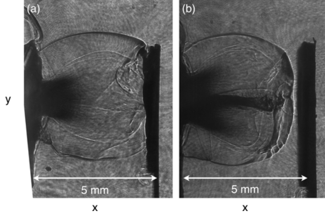
FIG. 3. Images of shadowgraphy taken at 20 ns from the laser timing. (a) Without offset ( d = 0 mm). (b) With offset ( d = 1 mm).
