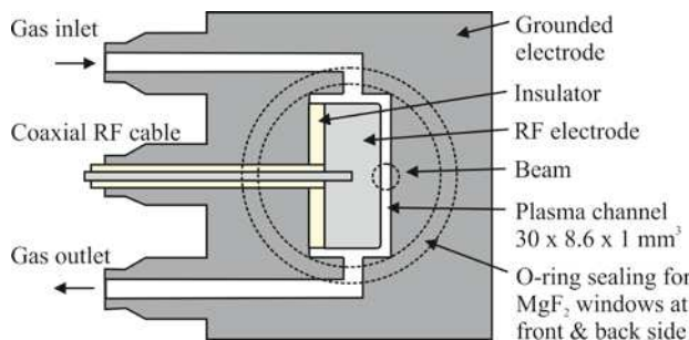
Fig. 1. Plasma source used for the absorption measurements. The absorption length used for the calculations is l = 8.6 mm.
