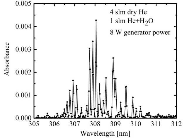
Fig. 3. Typical spectrum of the OH\ X^2\Pi(v''=0) \rightarrow A^2\Sigma^+(v'=0) transition. Dots indicate measured points. The total He flow is 5 slm of which 1 slm goes through the bubbler. The generator power is 8 W and the corresponding OH density n_{OH} = 2.64 \cdot 10^{20} \text{ m}^{-3} .
