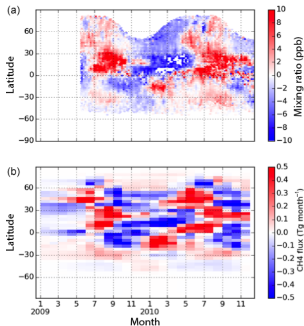
Figure 6. (a) Zonally averaged differences in CH 4 column mixing ratio between the two X\text{CH}_4^{\text{proxy}} retrievals ( X\text{CH}_4^{\text{ma}} - X\text{CH}_4^{\text{ct}} ). (b) Corresponding differences in a posteriori CH 4 flux between the proxy inversions using these data (PR-MA minus PR-CT).
