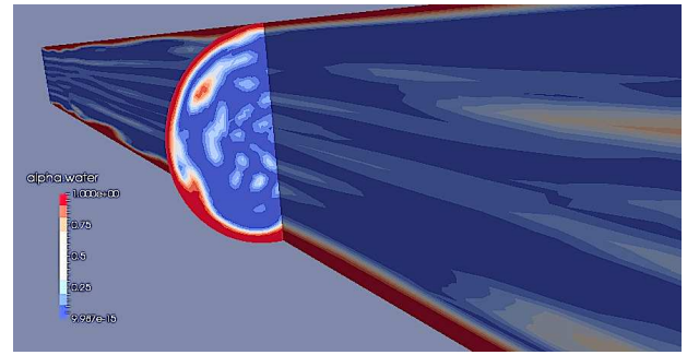
Figure 6 Fully developed annular flow regime
