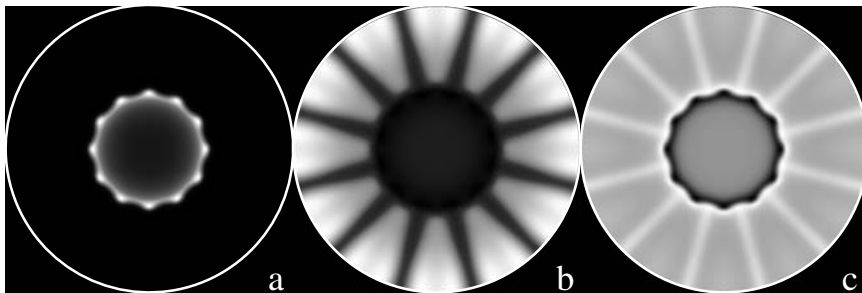
Figure 4. The surface structure of a cylindrical solution forms striations similar to sunspot penumbra. Here we display the (a) vertical magnetic field, (b) temperature and (c) density for a steady solution with R_a = 100,000 and Q = 64 .
