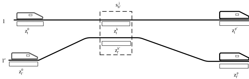
Fig. 6. The transfer station s_{ll'}^j .
