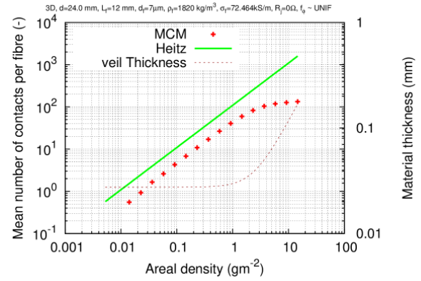
Figure 9. Material thickness and number of contacts per fibre for 3D isotropic (MCM) material compared with the 2D case (Heitz).
