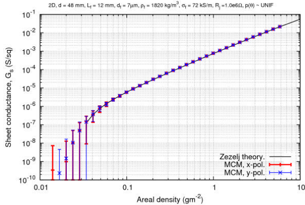
Figure 5. Effect of 1 MΩ contact resistance on veil with uniform fibre distribution.
