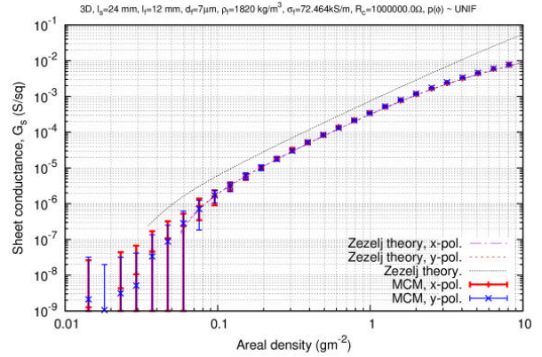
Figure 10. 3D veil with 1 \text{ M}\Omega contact resistance and uniform fibre distribution.
