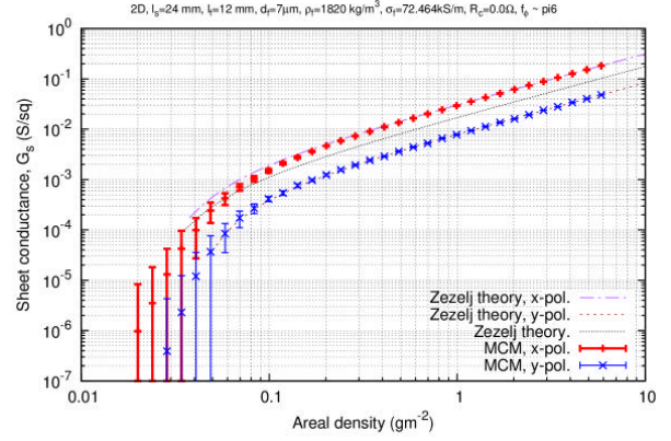
Figure 6. Sheet conductivity v areal density for truncated Gaussian fibre angular distribution – 90 \leq \varphi \leq 90 deg., with \sigma = 30 deg.
