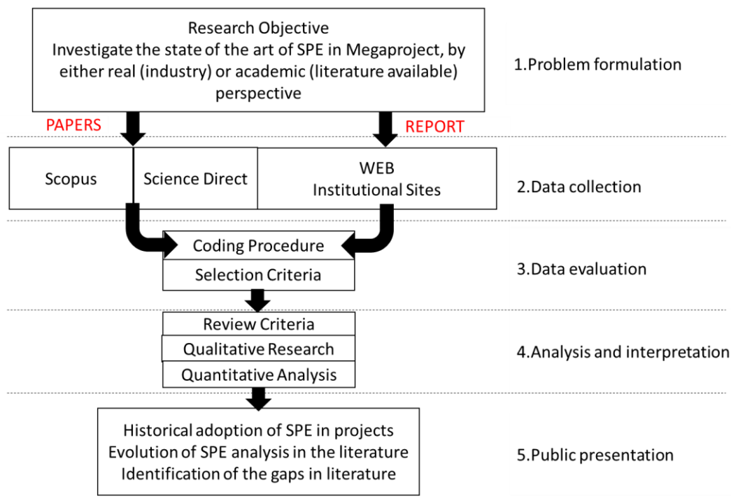
Fig. 3: Methodology Phases
