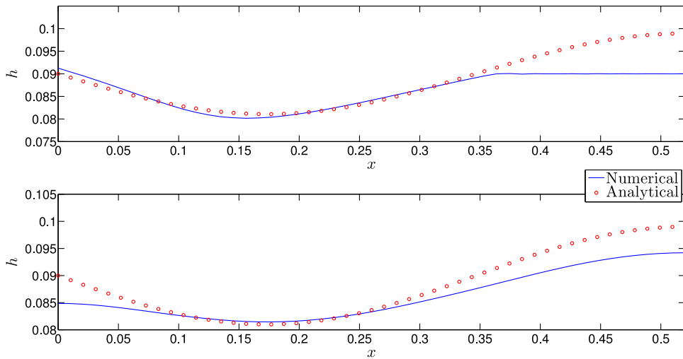
Fig. 5. Effect of surface tension on the free surface h(x, t) . The nonlinear forced shallow water equations are solved with parameter values L = 0.52, h_0 = 0.09, \gamma = 0, m = 1, q = 0.0027, T = 1.73 . Solid lines represent numerical solutions and circles correspond to exact solutions. Top panel: \sigma = 0 ; both solutions are plotted at t = 0.67 sec (see also video h_fromrest_nosigma.avi ). Bottom panel: \sigma = 0.027 ; the two solutions are shown at t = 0.36 sec (see also video h_fromrest_sigma.avi ).
