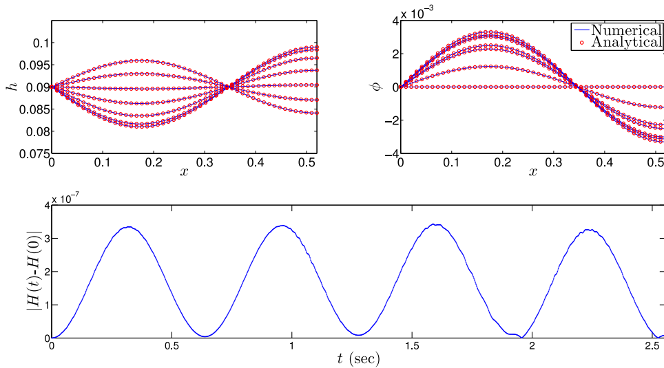
Fig. 4. Comparison between numerical solution and the exact standing wave solution in Eq. (15) of the linearised driven shallow water equations. Snapshots of the solutions of h(x, t) (top left panel) and \phi(x, t) (top right panel) are portrayed at t = 0.0, 0.08, 0.16, 0.23, 0.31, 0.39, 0.46 sec (see also videos h_flux.avi and phi_flux.avi ). Solid lines represent numerical solutions and circles correspond to exact solutions. The parameter values used are L = 0.52, h_0 = 0.09, \sigma = 0, \gamma = 0, m = 1, q = 0.0027, T = 4.62 . The relative energy |H(t) - H(0)| can be seen in the bottom panel, in dimensional units.
