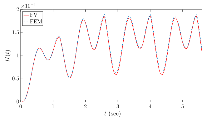
Fig. 8. Dimensional energy H(t) for the Hele-Shaw simulations with F = 0.7042 Hz. The energy plotted with dashed line corresponds to the finite element method (FEM), while the one with solid line to the finite volume method (FV).
