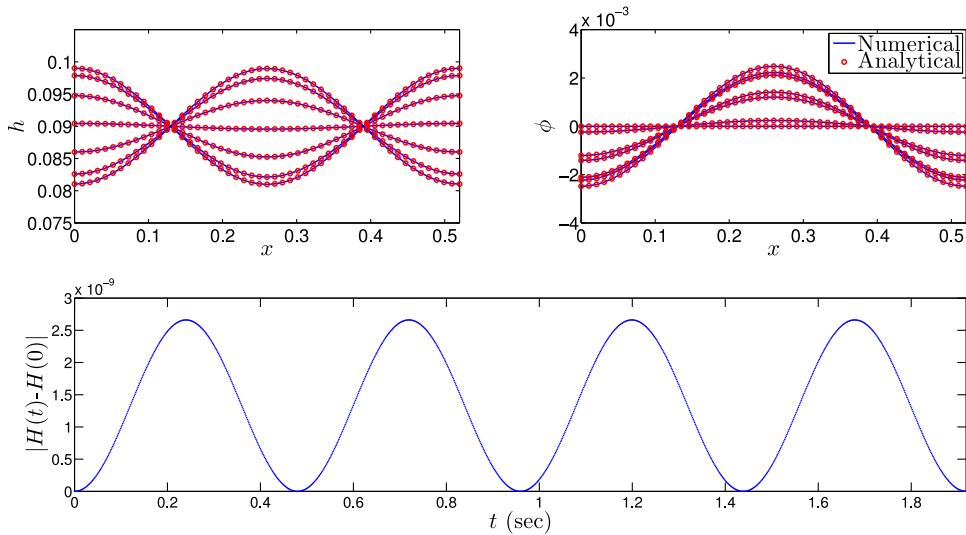
Fig. 2. Comparison between numerical solution and the exact standing wave solution in Eq. (13) of the linearised shallow water equations. Snapshots of the solutions of h(x, t) (top left panel) and \phi(x, t) (top right panel) are portrayed at t = 0.0, 0.08, 0.16, 0.23, 0.31, 0.39, 0.46 sec (see also videos h_exact.avi and phi_exact.avi ). Solid lines represent numerical solutions and circles correspond to exact solutions. The parameter values used are L = 0.52, h_0 = 0.09, \sigma = 0, \gamma = 0, m = 2, A = 0.009, T = 3.47 . The relative energy |H(t) - H(0)| is plotted in the bottom panel, in dimensional units.
