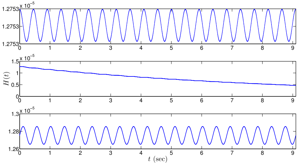
Fig. 3. Hamiltonian of the solution without/with damping (in dimensional units). Top panel: conservation of energy for linear undamped waves with \gamma = 0 . Middle panel: energy dissipation for linear damped waves with \gamma = 0.058 (Hamiltonian computed without factor e^{\gamma t} ). Bottom panel: energy conservation for linear damped waves with \gamma = 0.058 (Hamiltonian computed with factor e^{\gamma t} , as in (12)).
