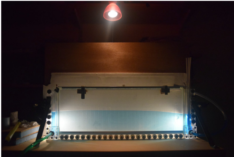
Fig. 1. Laboratory set-up of the Hele-Shaw cell used in the experiments. The water is highlighted with blue dye. In the middle section, water moves between two narrowly spaced glass plates, while on the left and right side two stilling wells are visible. The one on the left is connected via a hose to the pump, which is switched on and off periodically to create a wave. The hose on the right is open and not used for pumping. (For interpretation of the references to colour in this figure legend, the reader is referred to the web version of this article.)
