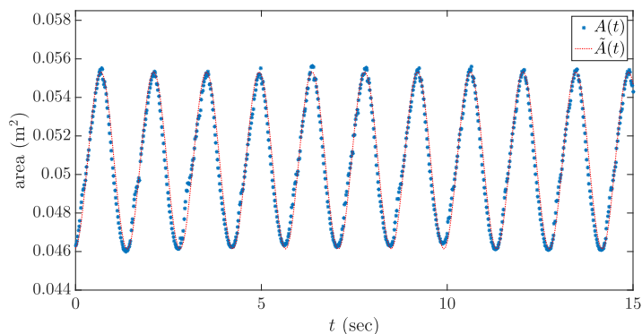
Fig. 6. Variation of the displaced area of water defined by the free surface over time (stars). The wave frequency is F = 0.7042 Hz and the corresponding initial water level is H_0 = 8.9 cm. We also superimpose a sinusoidal function (dotted line) defined by \hat{A}(t) = A_0 \sin(2\pi Ft - \frac{\pi}{2}) , where the amplitude A_0 = 0.0046 m 2 is calculated as half the distance from trough to crest.
