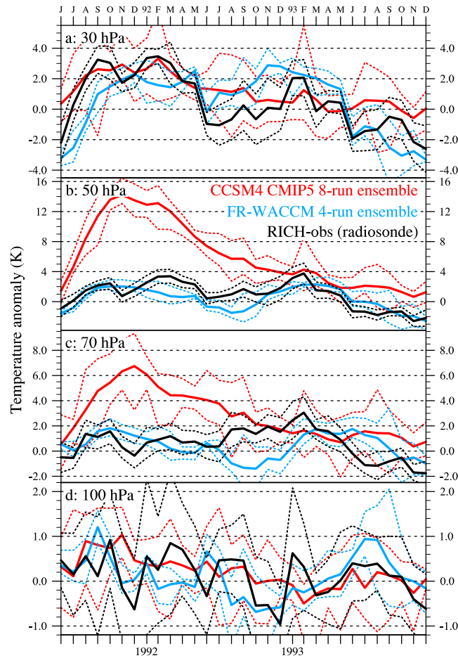
Figure 2. Post-Pinatubo monthly average stratospheric tropical (20°S–20°N) temperature anomalies are shown with respect to corresponding monthly mean values for June 1990–May 1991. Global radiosonde temperature observations compiled with the Radiosonde Innovation Composite Homogenization (RICH-obs) software package [Haimberger et al., 2012] are shown in black. Solid black lines show the average, and dashed black lines show the standard deviation, of the gridded observations. Corresponding tropical temperature anomalies from an ensemble of four FR-WACCM simulations with historical SSTs are shown in blue. Tropical temperatures from an ensemble of eight CMIP5 runs using CCSM4 with prescribed volcanic aerosols are shown in red. Solid lines show ensemble averages; dashed lines show ensemble maxima and minima monthly average anomalies.
