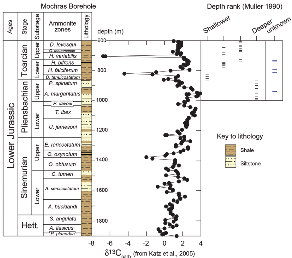
Figure 6. Carbon-isotope profile from bulk carbonate and palaeodepth changes inferred from benthic foraminifers. Modified after van de Schootbrugge et al. (2005). Hett. = Hettangian.
