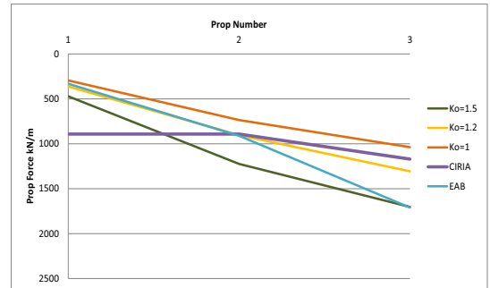
Figure 6. Maximum Prop Loads from empirical and numerical methods with varying K_0 for supported excavation with 3 prop levels
