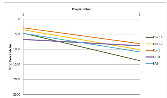
Figure 7. Maximum Prop Loads from empirical and numerical methods with varying K_0 for supported excavation with 2 prop levels
