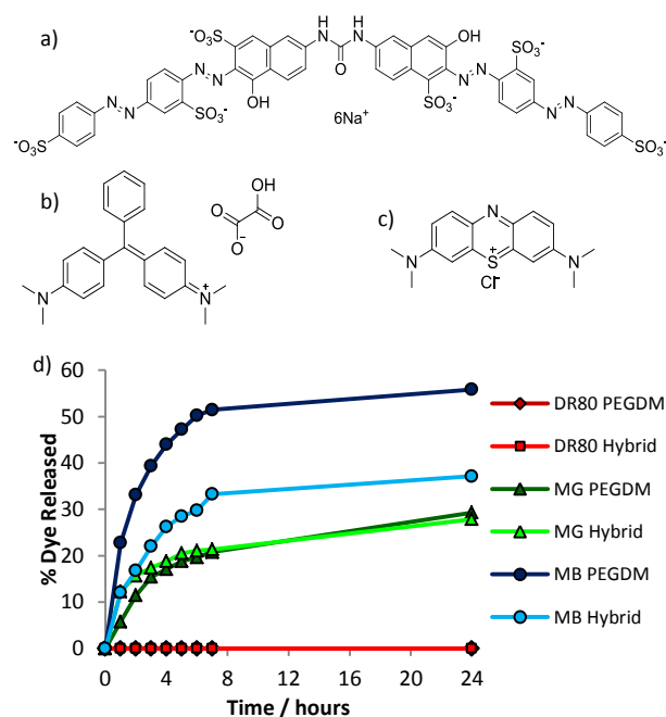
Figure 5. Structures of dyes (a) Direct Red 80, (b) malachite green oxalate, and (c) methylene blue chloride. A comparison of percentages of dye released from both PEGDM and hybrid gels in pH 7 buffer solution is shown in (d).
