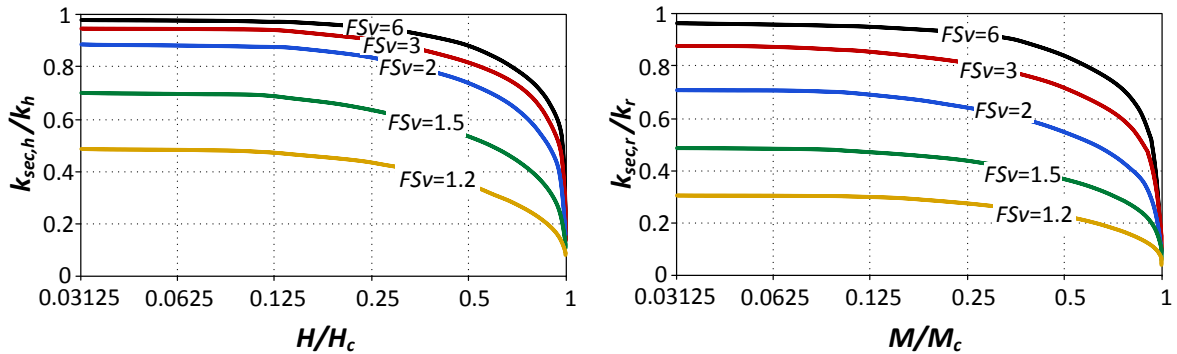
Fig. 10. Variation of secant foundation stiffness with mobilized foundation load level.
