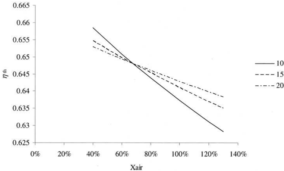
Fig. 5 Effect of excess air on thermal efficiency for various turndown ratios at U_{cap} = 0.1 ( U_c = 0.3 , T_{flF} = 450\text{ }^\circ\text{C} )
