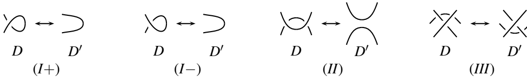
Figure 2: Reidemeister moves
