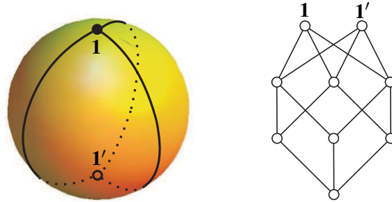
Figure 1: Regular CW complex X (left) with cell poset \mathbf{Q}_A (right) for |A| = 3 .
